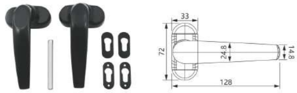
HL-01 Material: Aluminum alloy Finish: Powder coating, Oil injection Colour: Black, White, Silver, Brown, Beige, Champagne
