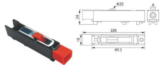
WW-95-D (R40) Material: Iron Finish: Color zinc plating Wheel Size: \Phi 20mm
