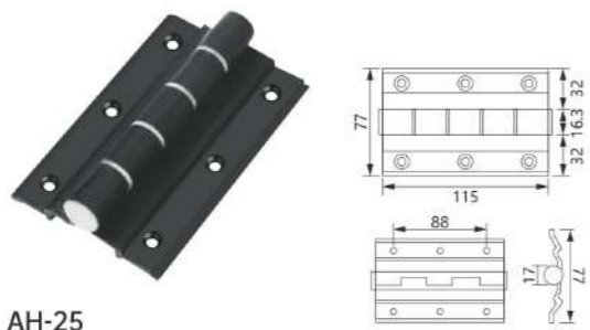
AH-25 Material: Aluminum Finish: Powder coating, Oil injection, Oxidation Colour: Black, White, Silver, Brown, Beige, Champagne
