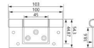
AH-19 Material: Aluminum Finish: Powder coating, Oil injection, Oxidation Colour: Black, White, Silver, Brown, Beige, Champagne, Charcoal
