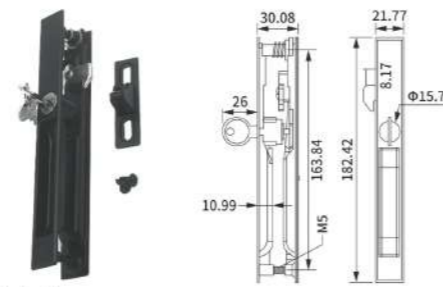
WL-13 (with key) Material: Aluminum alloy Finish: Powder coating, Oil injection Colour: Black, White, Silver, Beige
