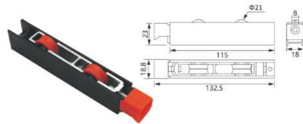
WW-95-D (R42) Material: Iron Finish: Color zinc plating Wheel Size: \Phi 21mm
