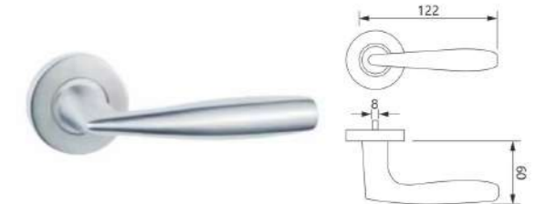
CY-38 (Solid handle) Material: Stainless steel 201/304 Finish: Satin
