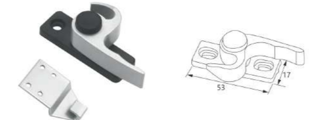
CL-09 (with aluminum hook) Material: Aluminum + Plastic Finish: Powder coating, Oil injection, Anodized Colour: Black, White, Silver, Brown, Beige
