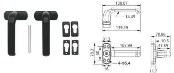
HL-09D Material: Aluminum alloy Finish: Powder coating, Oil injection Colour: Black, White, Silver, Brown, Beige, Champagne
