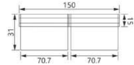
AH-09 Material: Aluminum Finish: Powder coating, Oil injection, Oxidation Colour: Black, White, Silver, Brown, Beige, Champagne
