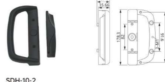
SDH-10-2 Material: Zinc alloy Finish: Powder coating, Oil injection Colour: Black, White, Silver
