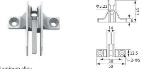
CF-17 Material: Aluminum alloy
