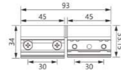
AH-13 Material: Aluminum Finish: Powder coating, Oil injection, Oxidation Colour: Black, White, Silver, Brown, Beige, Champagne
