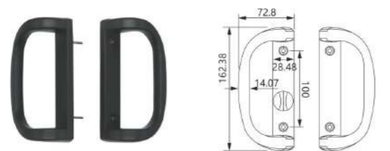
SDH-18-7 (604) Material: Aluminum alloy Finish: Powder coating, Oil injection Colour: Black, White, Silver
