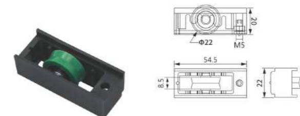
WW-48 Material: Plastic Wheel Size: \Phi 22mm
