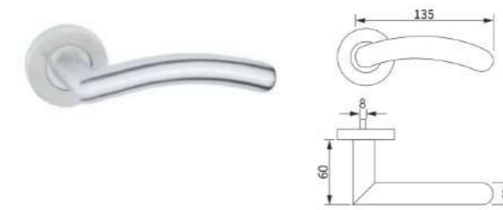
CY-08-1 Material: Stainless steel 201/304 Finish: Satin
