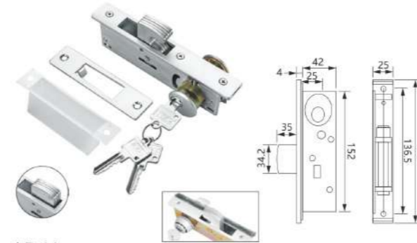
LB-14 Material: Iron body + Aluminum panel
