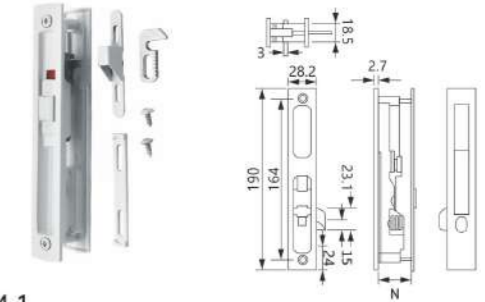
WL-24-1 Material: Aluminum alloy Finish: Powder coating, Oil injection Colour: Black, White, Silver, Beige
