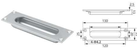
SDH-24 Material: Aluminum Finish: Powder coating, Oil injection Colour: Black, White, Silver
