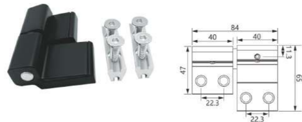
AH-27 (HL-6015) Material: Aluminum Finish: Powder coating, Oil injection, Oxidation Colour: Black, White, Silver, Brown, Beige, Champagne
