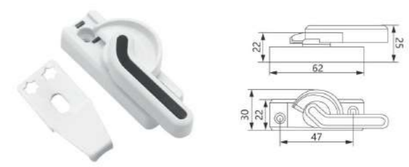
WH-05 (with iron hook) Material: Aluminum alloy Finish: Powder coating, Oil injection Colour: Black, White, Silver, Brown
