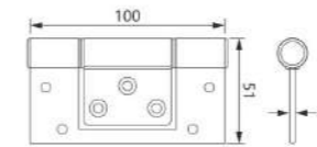
AH-18 Material: Aluminum Finish: Powder coating, Oil injection, Oxidation Colour: Black, White, Silver, Brown, Beige, Champagne
