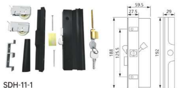
SDH-11-1 Material: Aluminum + Plastic Finish: Powder coating, Oil injection Colour: Black, White, Silver
