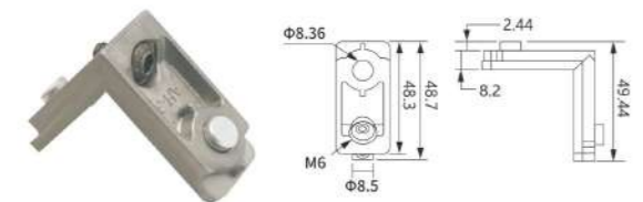
CF-01-3 Material: Aluminum alloy
