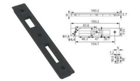
SDH-26 Material: Plastic Colour: Black, White, Silver
