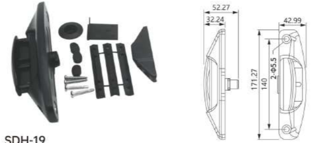
SDH-19 Material: Aluminum alloy Finish: Powder coating, Oil injection Colour: Black, White, Silver
