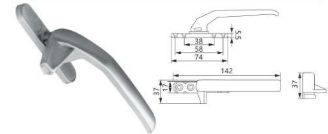
HL-26 (Plastic Type)
