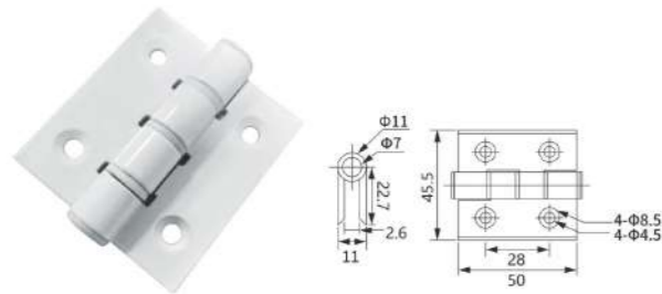
AH-39 Material: Aluminum Finish: Powder coating, Oil injection, Oxidation Colour: Black, White, Silver, Brown, Beige, Champagne
