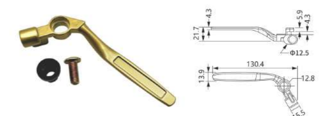
HL-83 Type: Left hand and right hand available Material: Aluminum alloy Finish: Powder coating, Oil injection Colour: Black, White, Silver, Brown, Beige, Champagne
