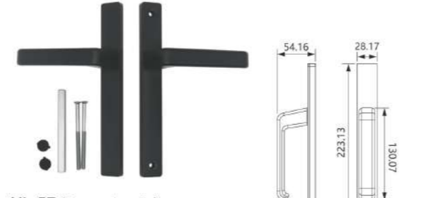
HL-57 (Dummy handle) Material: Aluminum alloy Finish: Powder coating, Oil injection Colour: Black, White, Silver, Brown, Beige, Champagne
