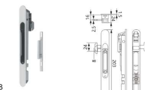
WL-28 Material: Aluminum Finish: Powder coating, Oil injection Colour: Black, White, Silver, Beige
