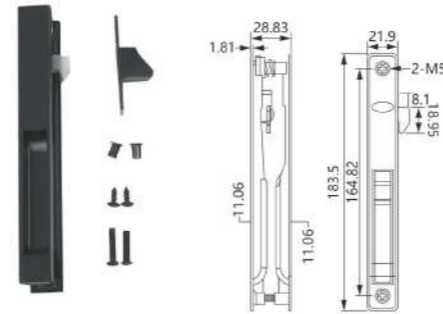
WL-12 Material: Aluminum alloy Finish: Powder coating, Oil injection Colour: Black, White, Silver, Beige
