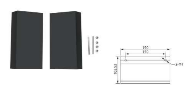
SDH-17-1 Material: Aluminum Finish: Powder coating, Oil injection Colour: Black, White, Silver, Brown, Beige, Champagne
