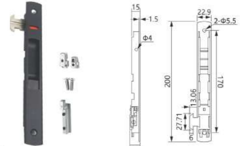
WL-27 Material: Aluminum Finish: Powder coating, Oil injection Colour: Black, White, Silver, Beige
