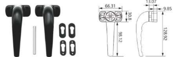
HL-03 Material: Zinc alloy Finish: Powder coating, Oil injection Colour: Black, White, Silver, Brown, Beige, Champagne
