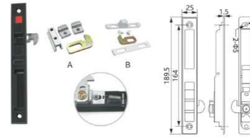
WL-21 (with spring/without spring) Material: Aluminum alloy Finish: Powder coating, Oil injection Colour: Black, White, Silver, Beige
