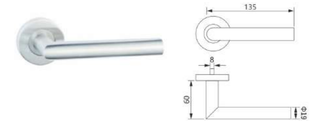
CY-22 Material: Stainless steel 201/304 Finish: Satin
