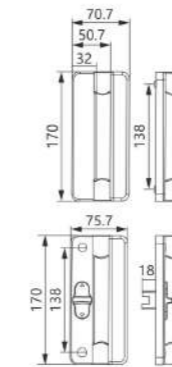
SDH-01 Material: Aluminum alloy/Zinc alloy Finish: Powder coating, Oil injection Colour: Black, White, Silver
