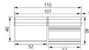
AH-20 Material: Aluminum Finish: Powder coating, Oil injection, Oxidation Colour: Black, White, Silver, Brown, Beige, Champagne
