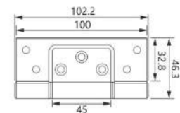
AH-22 (Iron pin) Material: Aluminum Finish: Powder coating, Oil injection, Oxidation Colour: Black, White, Silver, Brown, Beige, Champagne, Charcoal
