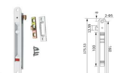
WL-29 Material: Aluminum Finish: Powder coating, Oil injection Colour: Black, White, Silver, Beige
