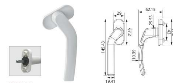
WH-34 Material: Aluminum alloy Finish: Powder coating, Oil injection Colour: Black, White, Silver, Brown, Beige
