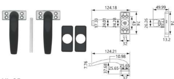
HL-05 Material: Aluminum alloy Finish: Powder coating, Oil injection Colour: Black, White, Silver, Brown, Beige, Champagne
