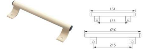
HL-46 Material: Aluminum Size: 7" / 10" Finish: Powder coating, Oil injection Colour: Black, White, Silver, Brown, Beige, Champagne
