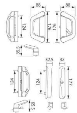
SDH-06 Material: Aluminum alloy + Zinc alloy Finish: Powder coating, Oil injection Colour: Black, White, Silver
