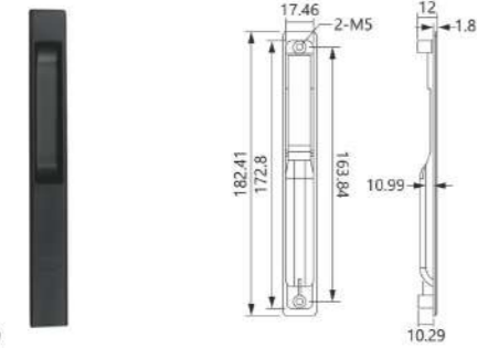
WL-09 Material: Aluminum alloy Finish: Powder coating, Oil injection Colour: Black, White, Silver, Beige
