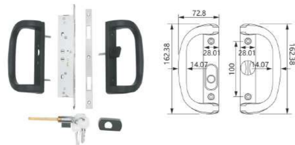
SDH-18-5 (602) (with keys) Material: Aluminum alloy Finish: Powder coating, Oil injection Colour: Black, White, Silver
