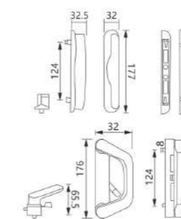
SDH-14 Material: Aluminum alloy/Zinc alloy Finish: Powder coating, Oil injection Colour: Black, White, Silver
