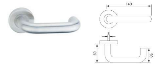
CY-21 Material: Stainless steel 201/304 Finish: Satin
