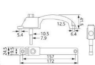
HL-39 Material: Aluminum alloy Finish: Powder coating, Oil injection Colour: Black, White, Silver, Brown, Beige, Champagne
