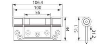
Intermediate hinge
