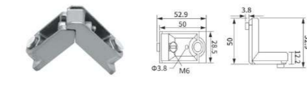
CF-16 Material: Aluminum alloy
