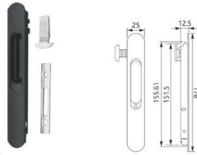
WL-08 Material: Aluminum Finish: Powder coating, Oil injection Colour: Black, White, Silver, Beige
