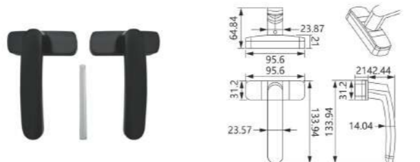
HL-09E Material: Aluminum alloy Finish: Powder coating, Oil injection Colour: Black, White, Silver, Brown, Beige, Champagne
