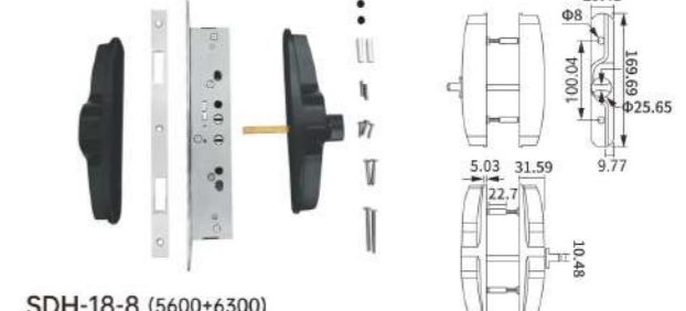
SDH-18-8 (5600+6300) Material: Aluminum alloy Finish: Powder coating, Oil injection Colour: Black, White, Silver
