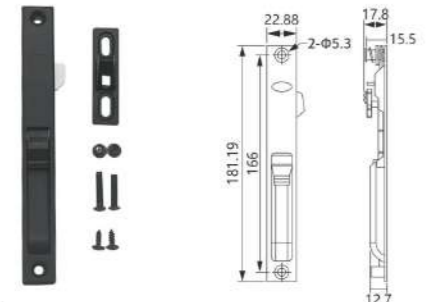
WL-10 Material: Aluminum alloy/Aluminum alloy + Plastic Finish: Powder coating, Oil injection Colour: Black, White, Silver, Beige
