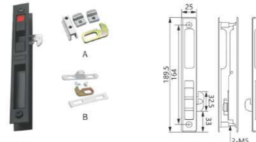
WL-22 Material: Aluminum alloy Finish: Powder coating, Oil injection Colour: Black, White, Silver, Beige
