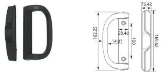
SDH-18-3 (606) Material: Aluminum alloy Finish: Powder coating, Oil injection Colour: Black, White, Silver
