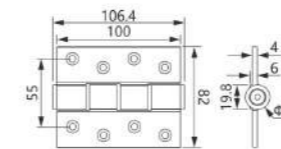
Intermediate hinge
