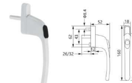
WH-03 Material: Aluminum alloy Finish: Powder coating, Oil injection Colour: Black, White, Silver, Brown, Beige
