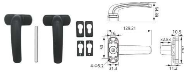
HL-09B Material: Aluminum alloy Finish: Powder coating, Oil injection Colour: Black, White, Silver, Brown, Beige, Champagne
