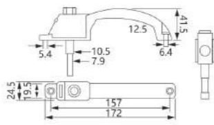
HL-38 Material: Aluminum alloy Finish: Powder coating, Oil injection Colour: Black, White, Silver, Brown, Beige, Champagne
