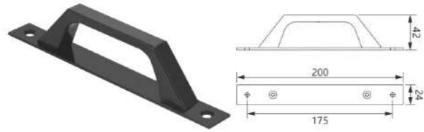
HL-49 Material: Aluminum Finish: Powder coating, Oil injection Colour: Black, White, Silver, Brown, Beige, Champagne
