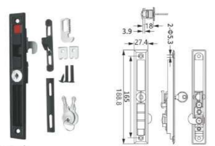
WL-19 (with key) Material: Zinc alloy Finish: Powder coating, Oil injection Colour: Black, White, Silver, Beige
