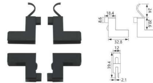
WW-87 (EBM) Material: Plastic
