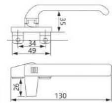
HL-40 Type: Left hand and right hand available Material: Aluminum alloy Finish: Powder coating, Oil injection Colour: Black, White, Silver, Brown, Beige, Champagne
