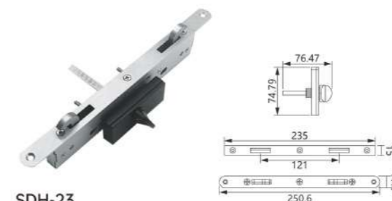
SDH-23 Material: Aluminum alloy Finish: Powder coating, Oil injection Colour: Black, White, Silver
