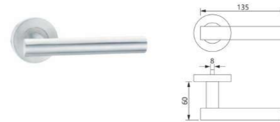
CY-08 Material: Stainless steel 201/304 Finish: Chrome
