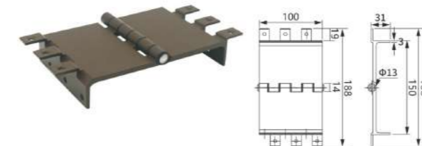
AH-45 Material: Aluminum Finish: Powder coating, Oil injection, Oxidation Colour: Black, White, Silver, Brown, Beige, Champagne, Charcoal
