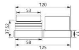
AH-14 Material: Aluminum Finish: Powder coating, Oil injection, Oxidation Colour: Black, White, Silver, Brown, Beige, Champagne
