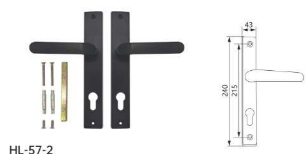
HL-57-2 Material: Iron plate + Aluminum alloy handle Finish: Powder coating Colour: Black, White, Silver, Brown, Beige, Champagne
