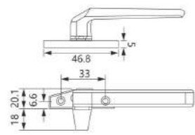
HL-31 Type: Left hand and right hand available Material: Aluminum alloy Finish: Powder coating, Oil injection Colour: Black, White, Silver, Brown, Beige, Champagne
