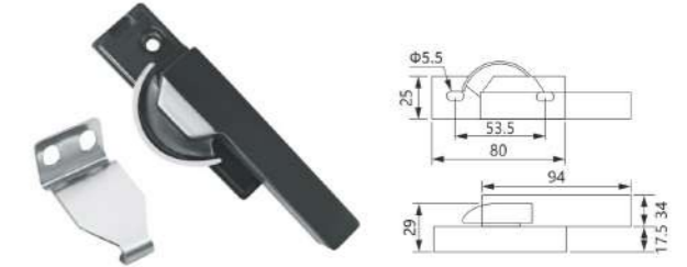
CL-13 (with SS201 hook) Material: Zinc alloy Finish: Powder coating, Oil injection Colour: Black, White, Silver, Brown
