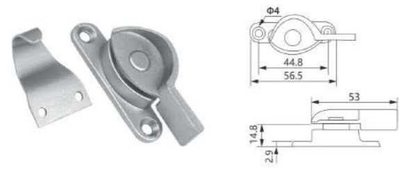
CL-01 Material: Aluminum alloy Finish: Powder coating, Oil injection Colour: Black, White, Silver, Brown
