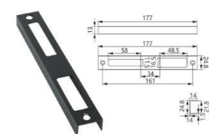
SDH-25 Material: Aluminum Finish: Powder coating, Oil injection Colour: Black, White, Silver
