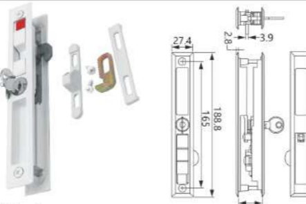
WL-20 (with key) Material: Zinc alloy Finish: Powder coating, Oil injection Colour: Black, White, Silver, Beige
