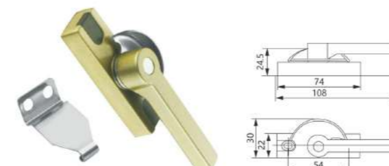
CL-10 (with SS201 hook) Material: Aluminum alloy/Zinc alloy Finish: Powder coating, Oil injection Colour: Black, White, Silver, Brown
