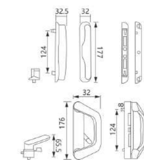
SDH-14-1 (with keys) Material: Aluminum alloy + Zinc alloy Finish: Powder coating, Oil injection Colour: Black, White, Silver
