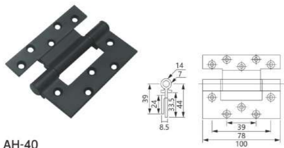
AH-40 Material: Aluminum Finish: Powder coating, Oil injection, Oxidation Colour: Black, White, Silver, Brown, Beige, Champagne
