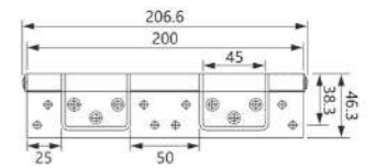
AH-24 Material: Aluminum Finish: Powder coating, Oil injection, Oxidation Colour: Black, White, Silver, Brown, Beige, Champagne, Charcoal
