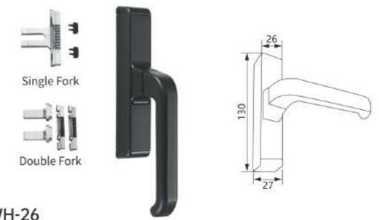
WH-26 Material: Zinc alloy bottom+Aluminum alloy handle/ All aluminum alloy Finish: Powder coating, Oil injection Colour: Black, White, Silver, Brown, Beige
