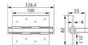
Hinge handle
