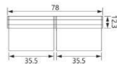
AH-12 Material: Aluminum Finish: Powder coating, Oil injection, Oxidation Colour: Black, White, Silver, Brown, Beige, Champagne
