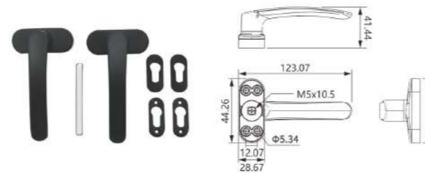
HL-09C Material: Aluminum alloy Finish: Powder coating, Oil injection Colour: Black, White, Silver, Brown, Beige, Champagne
