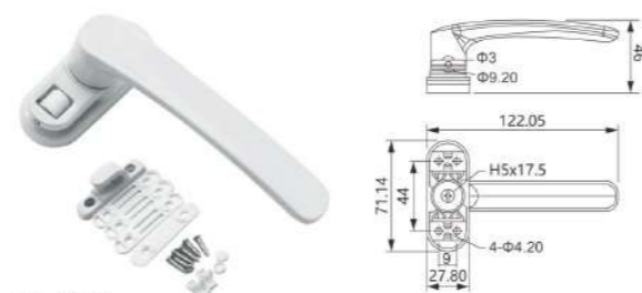
HL-42C Type: Left hand and right hand available Material: Aluminum alloy Finish: Powder coating, Oil injection Colour: Black, White, Silver, Brown, Beige, Champagne
