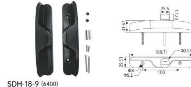
SDH-18-9 (6400) Material: Aluminum alloy Finish: Powder coating, Oil injection Colour: Black, White, Silver
