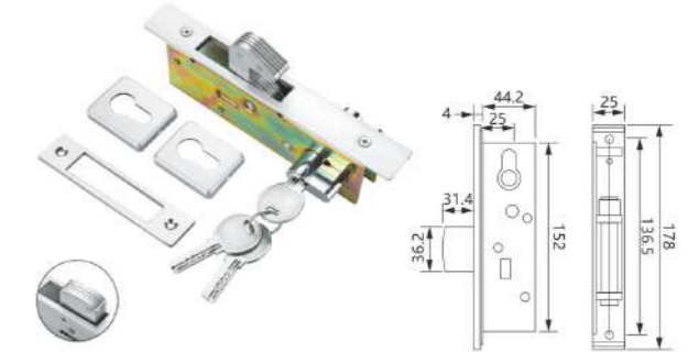
LB-14-1 (with normal cylinder) Material: Iron body + Aluminum panel
