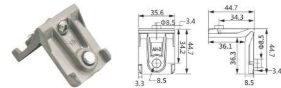
CF-01-2 Material: Aluminum alloy
