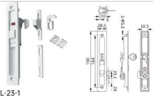
WL-23-1 Material: Aluminum alloy Finish: Powder coating, Oil injection Colour: Black, White, Silver, Beige
