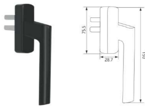
WH-18 Material: Aluminum alloy Finish: Powder coating, Oil injection Colour: Black, White, Silver, Brown, Beige, Champagne
