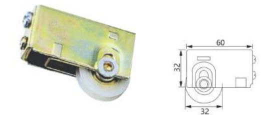
WW-09 Material: Iron Finish: Iron plated color galvanized Wheel Size: \Phi 32mm
