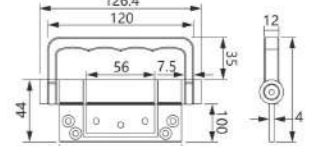
Hinge handle
