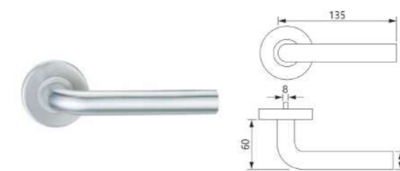
CY-20 Material: Stainless steel 201/304 Finish: Satin
