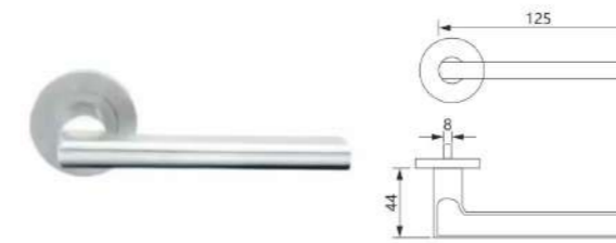
CY-09 Material: Stainless steel 201/304 Finish: Satin
