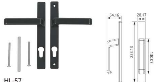
HL-57 Material: Aluminum alloy Finish: Powder coating, Oil injection Colour: Black, White, Silver, Brown, Beige, Champagne
